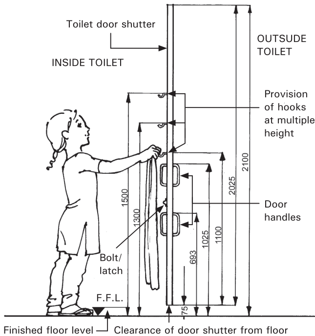
Drawing 2:24a. Section
