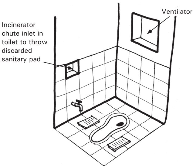
Drawing 2:37. Chute for Incinerator from Girl's Toilet
