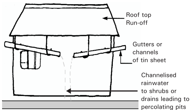
Drawing 2:35. Channelising roof top run off rainwater
