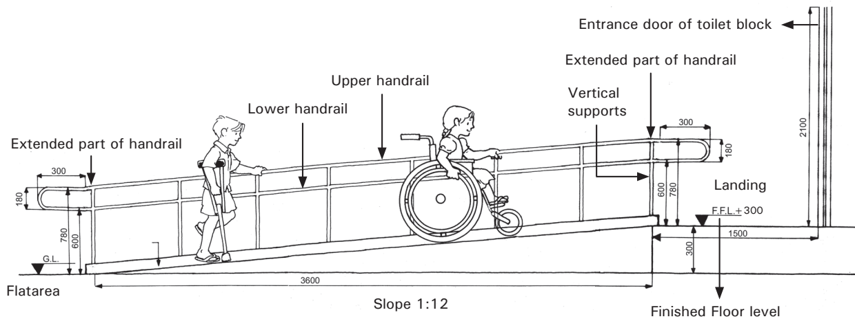
Drawing 2:17. Section
