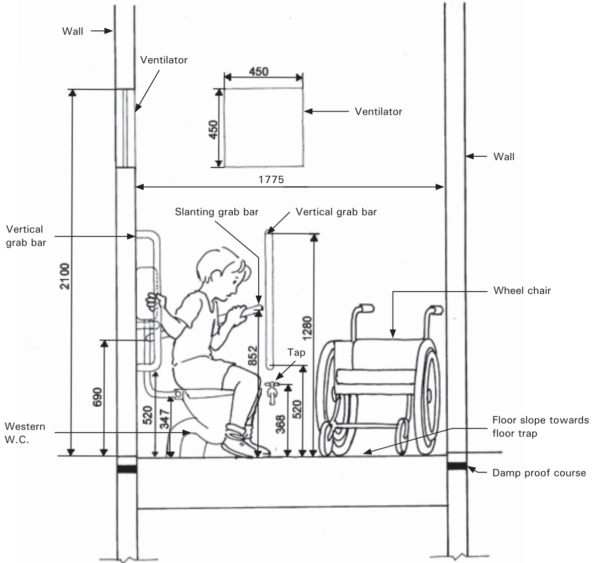
Drawing 2:21b. Section
