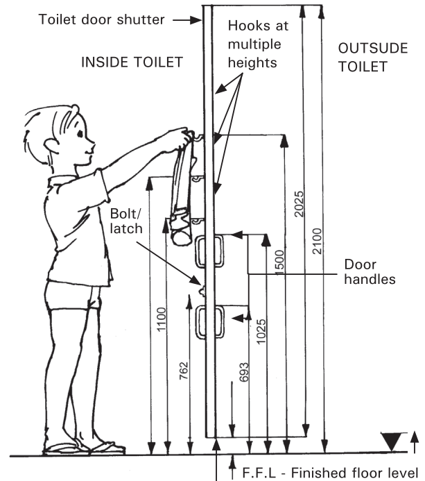
Drawing 2:24b. Section
