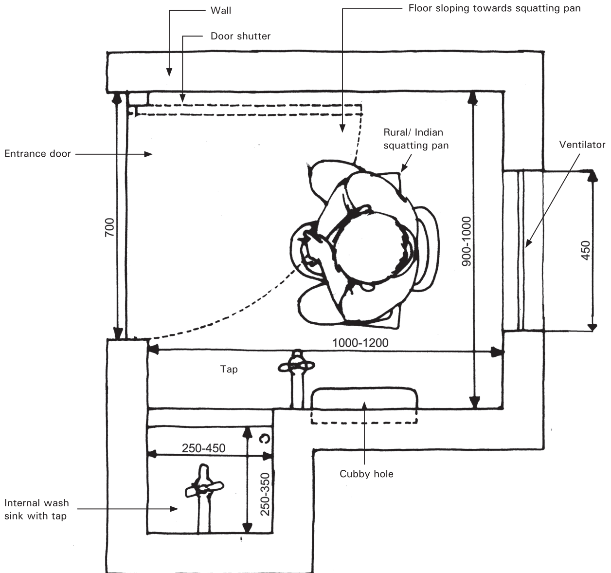
Drawing 2:23. Plan
