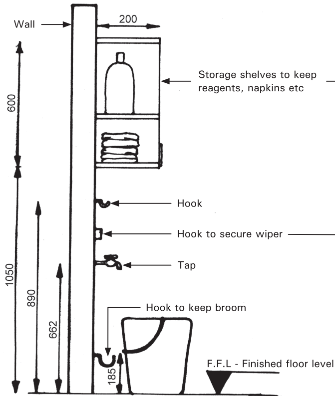
Drawing 2:29a. Section
