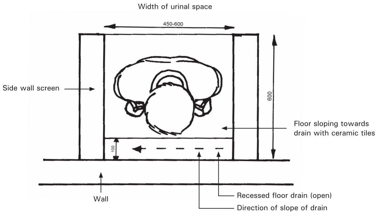
Drawing 2:19c. Plan
