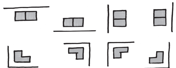
Drawing 2:4. Site planning of toilet blocks in different directions
