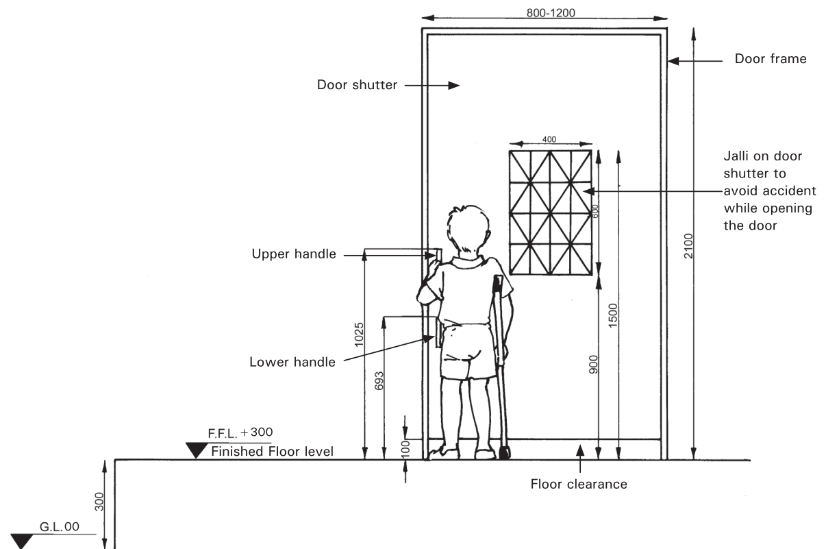
Drawing 2:18b. Provisions with crutches - Elevation
