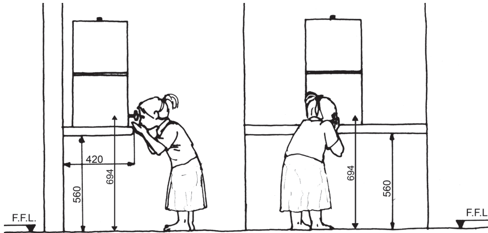
Drawing 2:28. Section & Elevation
