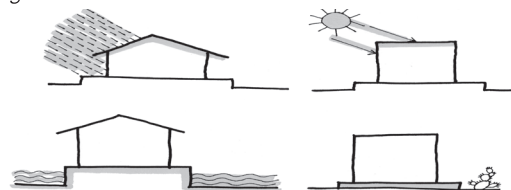
Drawing 2:16. Plinth wall and roof design as per local geo-climatic conditions
