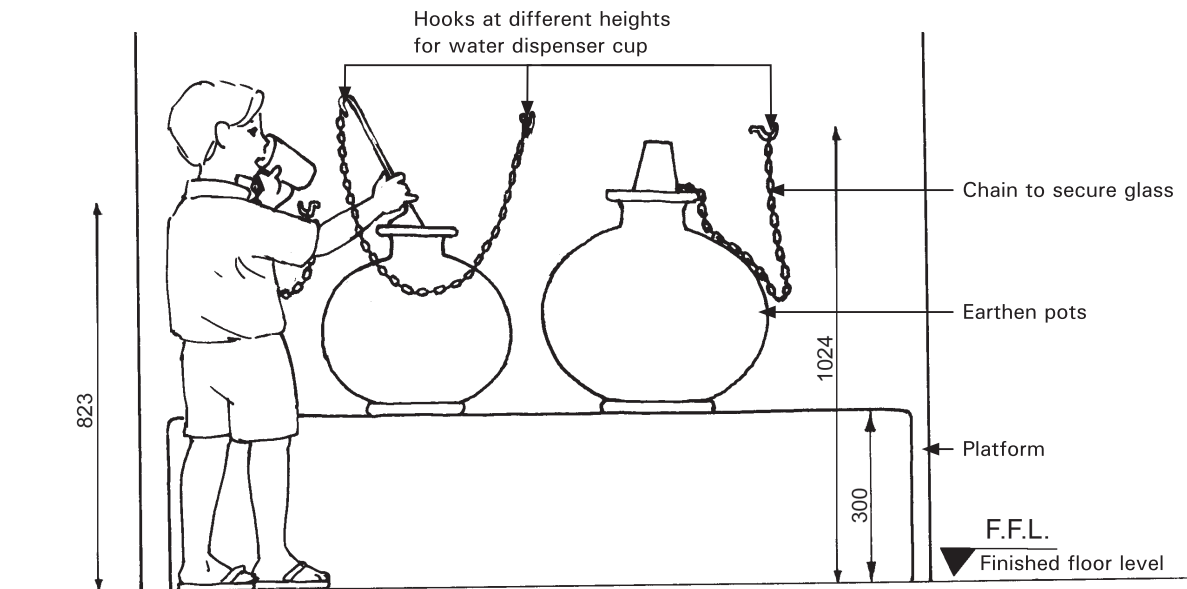
Drawing 2:27a. Elevation
