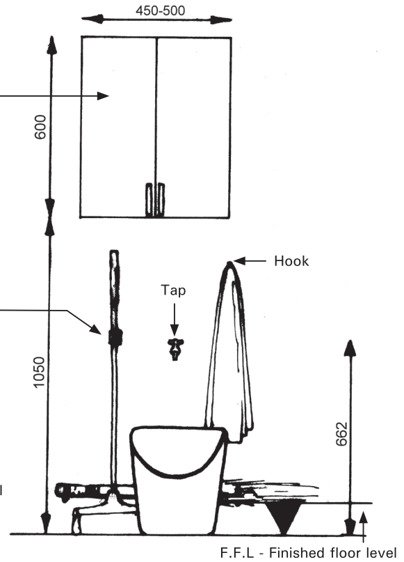
Drawing 2:29b. Elevation
