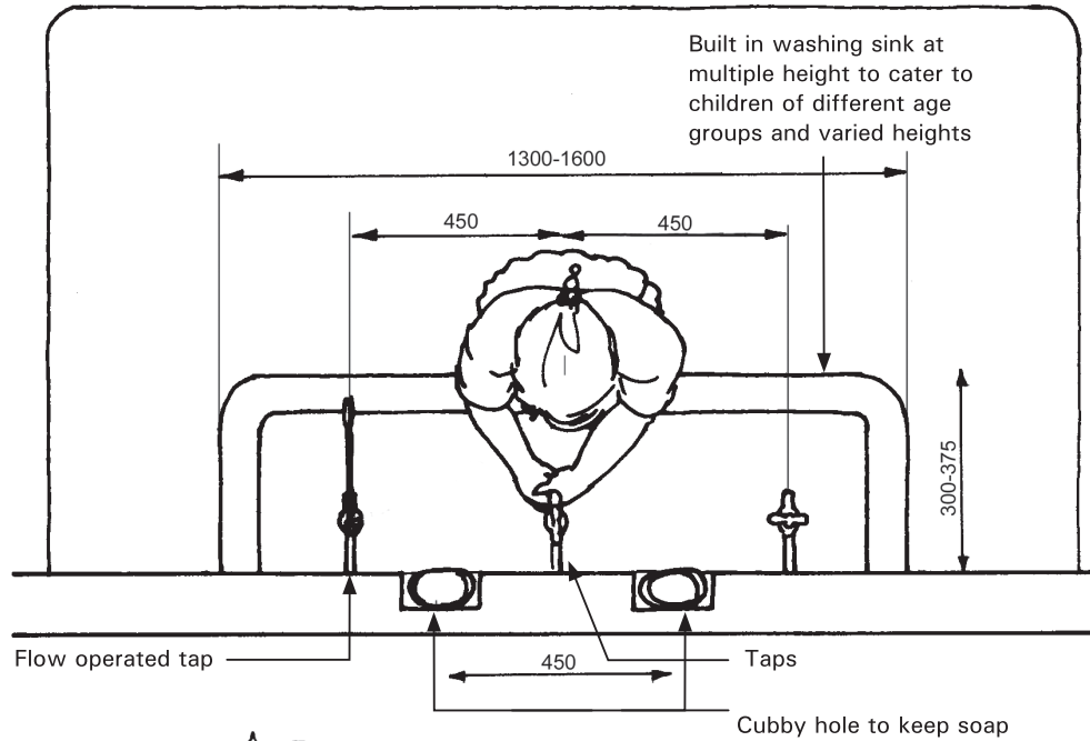
Drawing 2:26a. Plan
