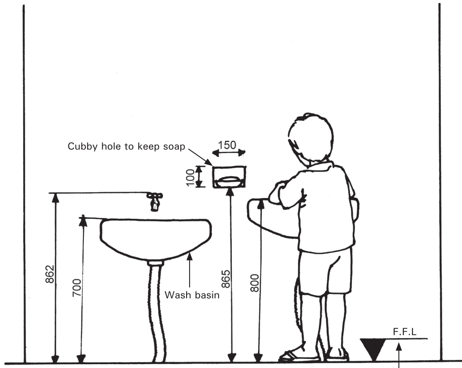
Drawing 2:25c. Elevation
