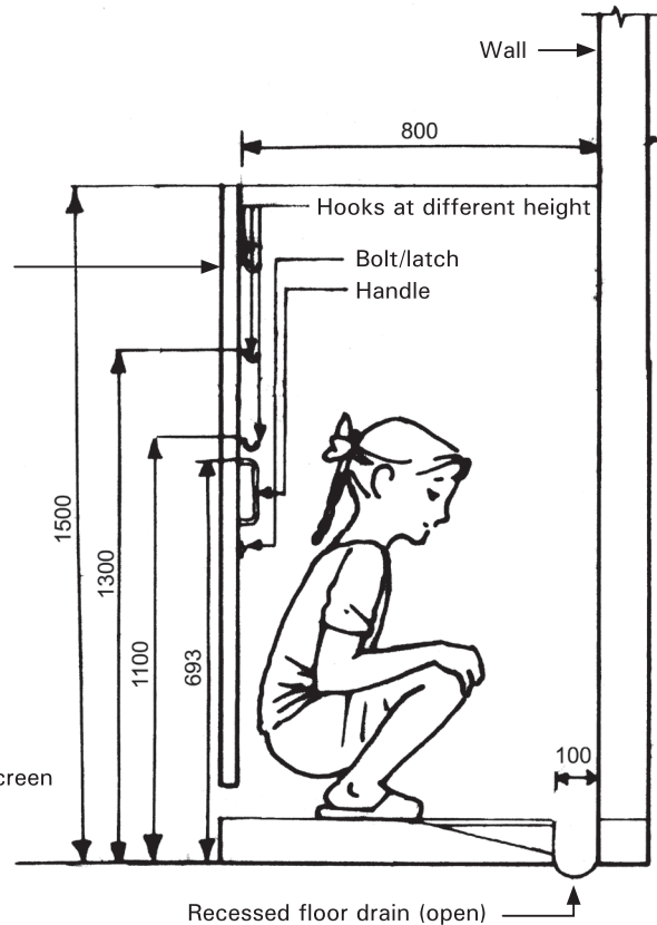
Drawing 2:19b. Section
