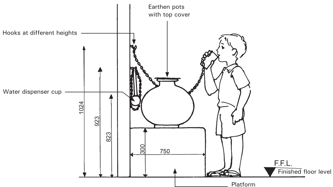
Drawing 2:27b. Section
