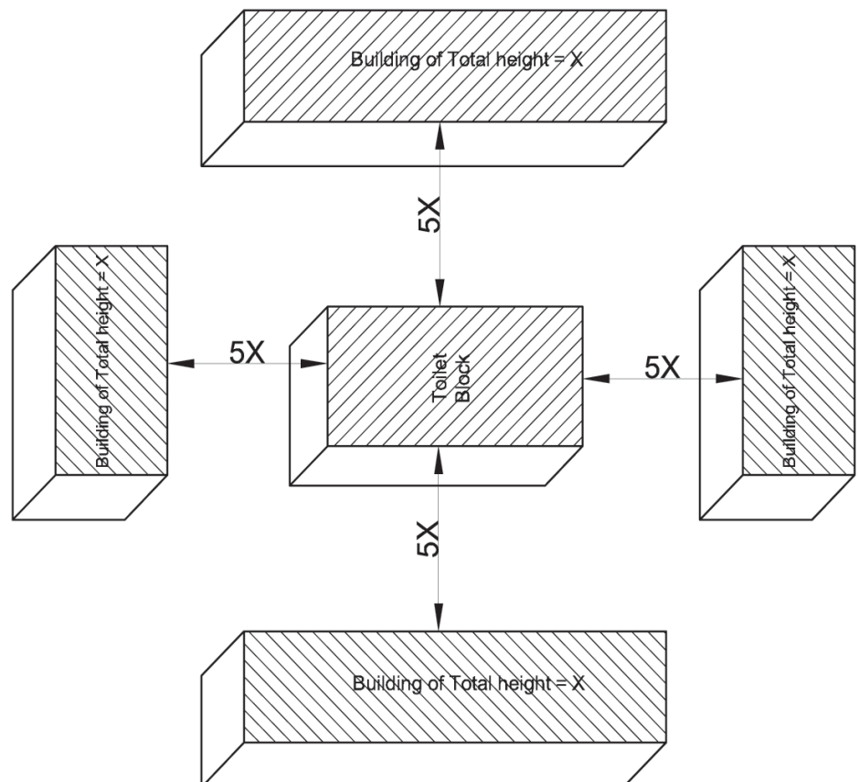
Drawing 2:31. Placement of building for Wind penetration
