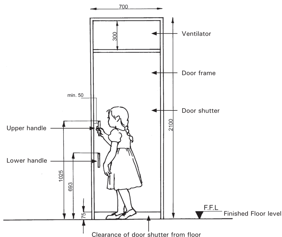
Drawing 2:18c. Elevation
