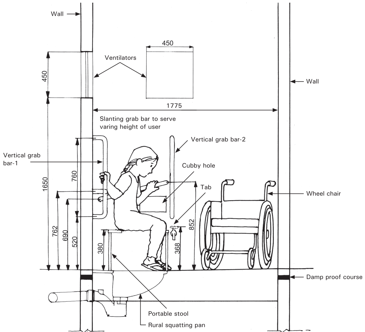
Drawing 2:20b. Section
