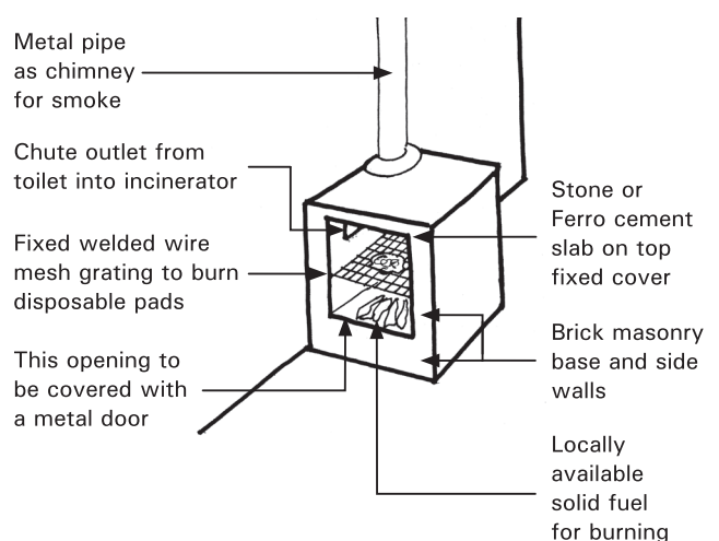
Drawing 2:36. Masonry incinerator outside girl's toilet
