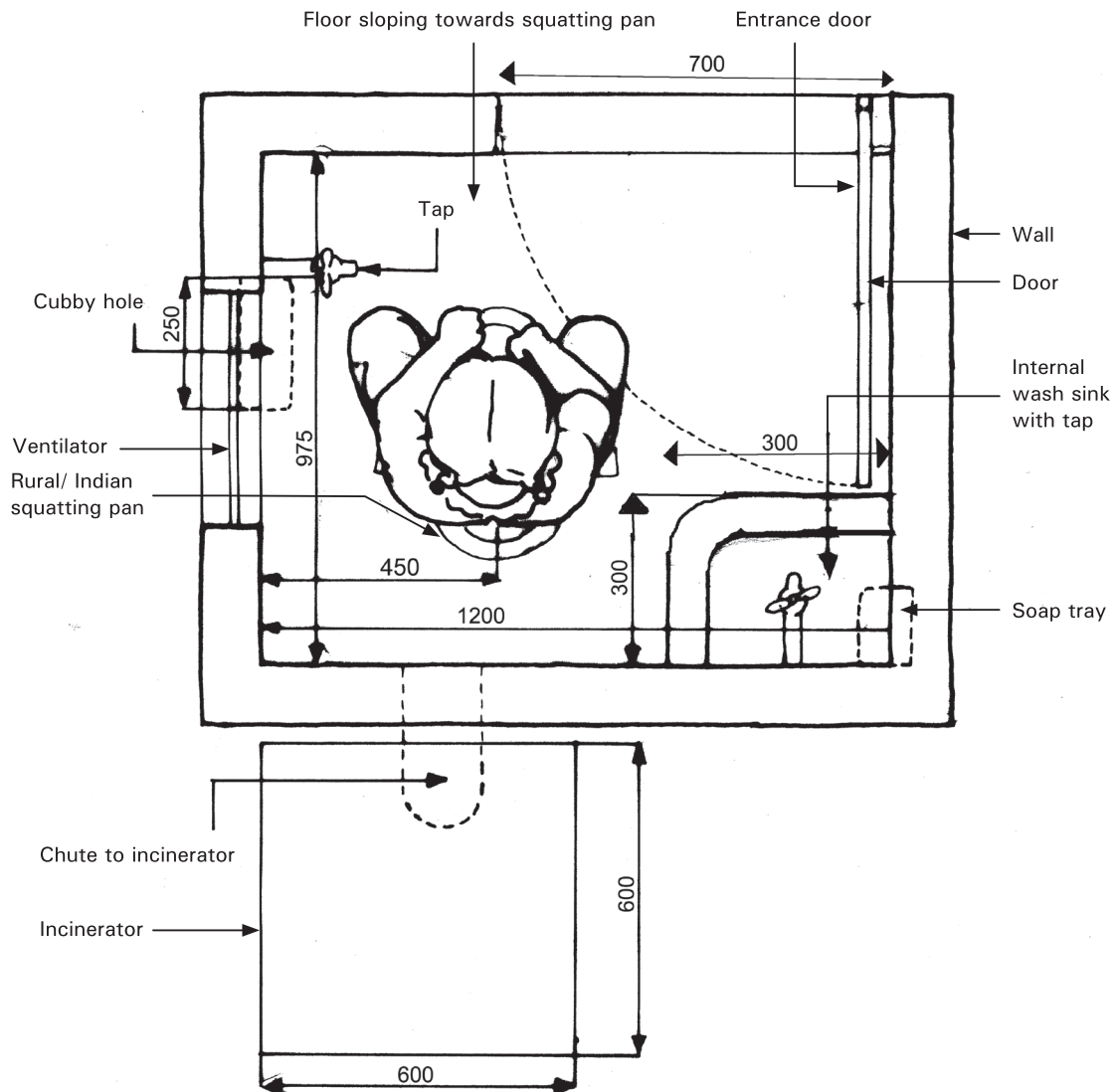
Drawing 2:22a. Plan
