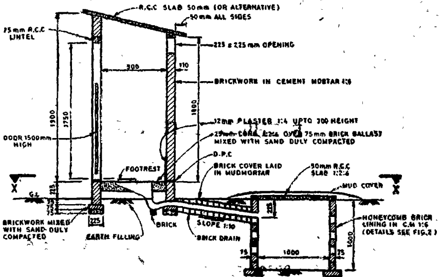
SIDE - VIEW SECTION.
