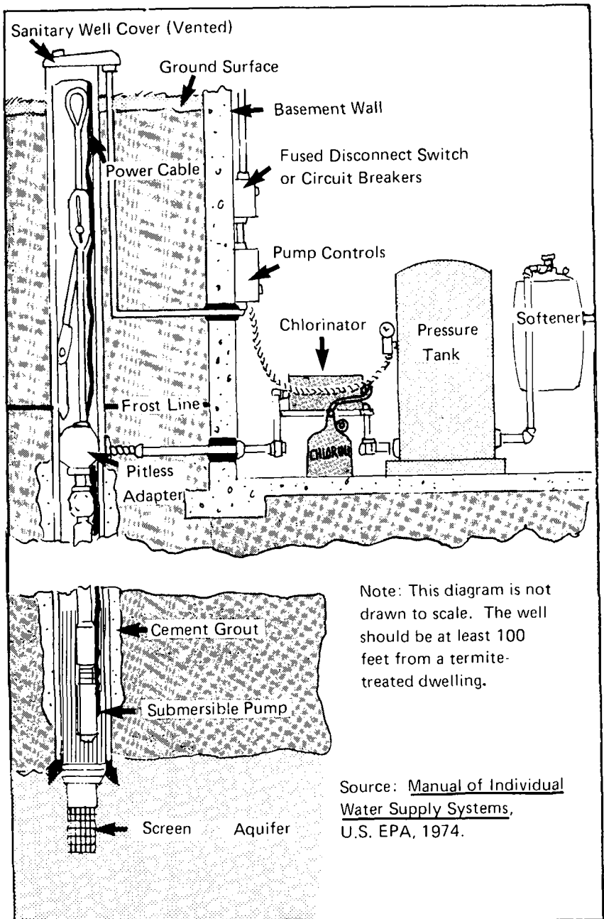
FIGURE 3 Water Is Pumped from a Domestic Well To Supply a Home Water System—Chlorinators and Water Softeners Are Used in Some Cases When Well Water needs Treatment before Consumption
