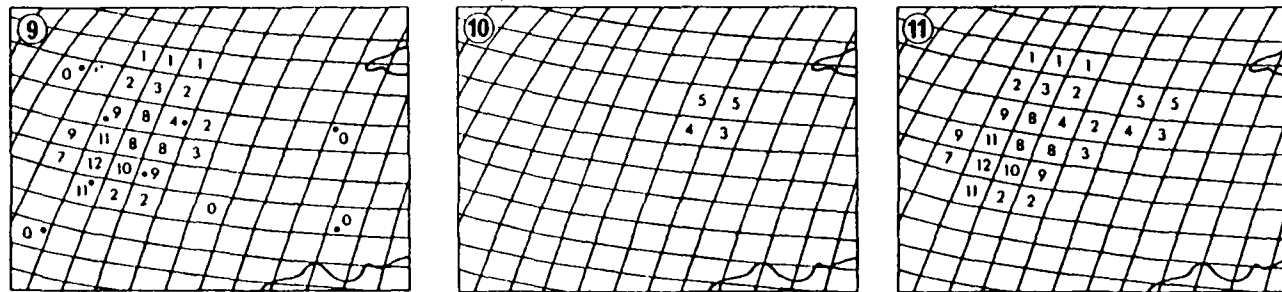
Fig. 12(b). A simulation of BIAS procedures on an interactive image processing screen. In (1) - (3) IR or VIS images are displayed for time (t), and compared with imagery for time (t+12) in (4). In (3) SYNOP reports for time (t+12) are superimposed, and in (4) rainfall totals are reduced by morphoclimatic weights. In (5) and (6), imagery for times (t) and (t+12) are analyzed for cloud type, and in (7) adjustments made for movement and/or development of clouds between those times. In (8) calibration station areas of influence are outlined. In (9), "meteorological entry" estimates of 12-hr rain are made where possible, and increased by the morphoclimatic weights. In (10) "climate entry" estimates are made for remaining rain-bearing product squares. (11) is the final 12-hr analysis.
