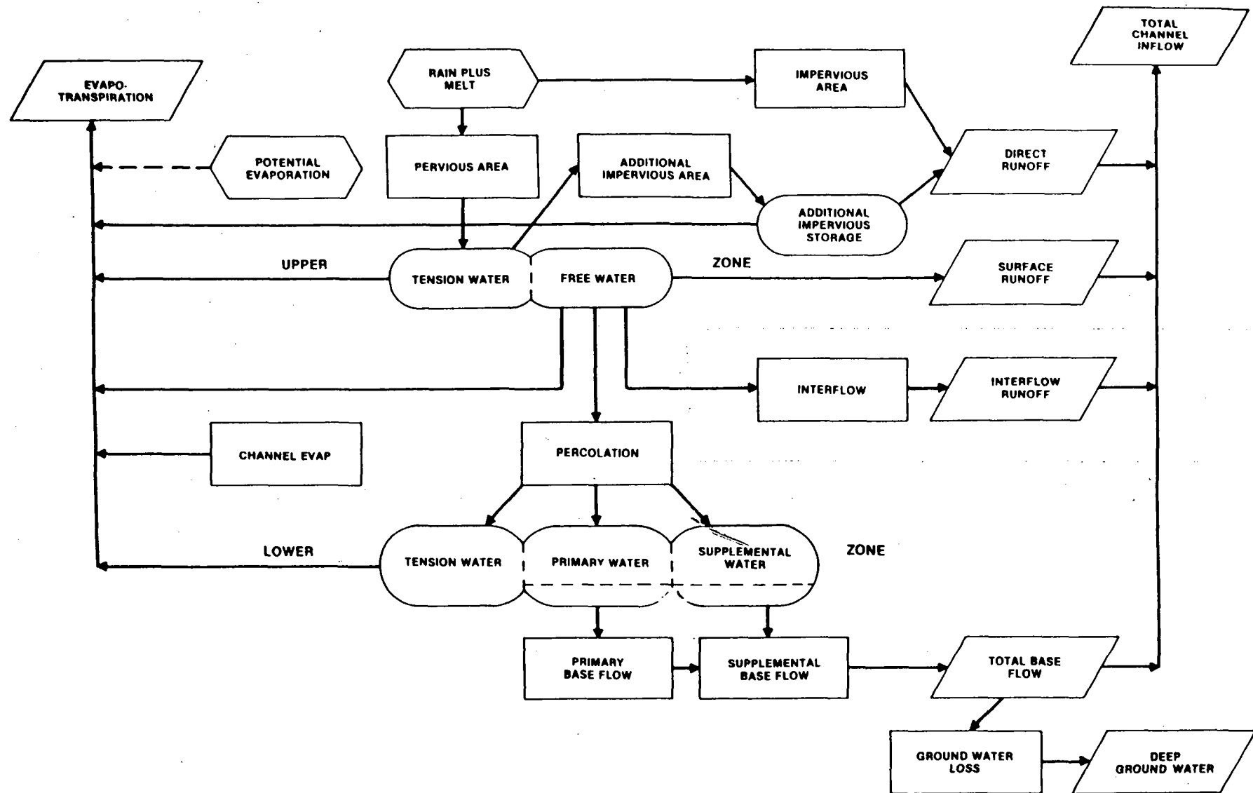
Fig. 22. National (United States) Weather Service River Forecast System (NWSRFS) Sacramento Soil Moisture Accounting Model schematic diagram (Peck et al., 1981).
