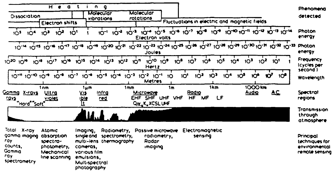
Fig. 1. The electromagnetic spectrum. The scales give the energy of the photons corresponding to radiation of different frequencies and wavelengths. The product of any wavelength and frequency is the speed of light. Phenomena detected at different wavelengths are shown with some of the principal associated techniques for environmental remote sensing. (From Barrett and Curtis, 1982.)
