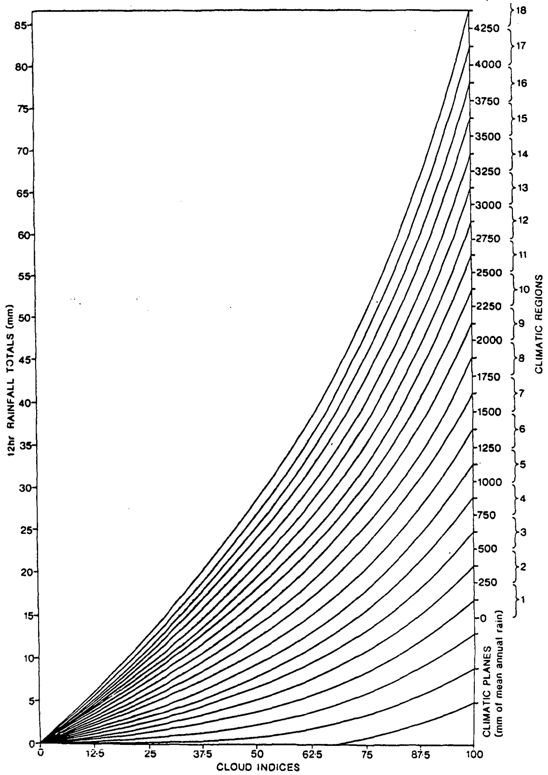
Fig. 13. THE BIAS "Global Regression" (Barrett, 1983b).
