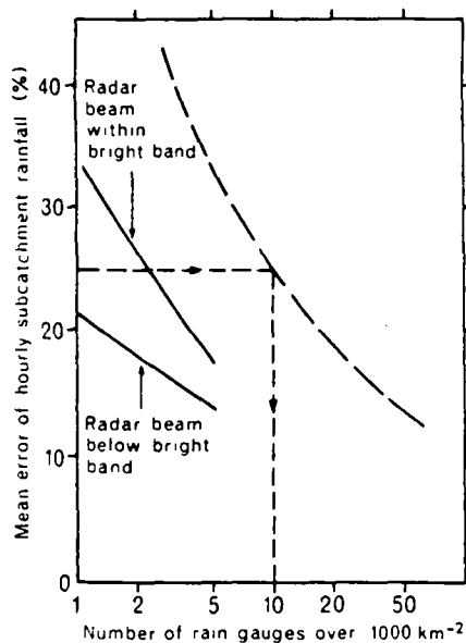
Fig. 11. Radar mean error versus density of calibrating rain gage sites (solid lines), and the mean error of hourly subcatchment totals for mean rainfall events in middle latitudes in the absence of radar (broken line). (From Barrett, 1980 after Browning, 1978.)
