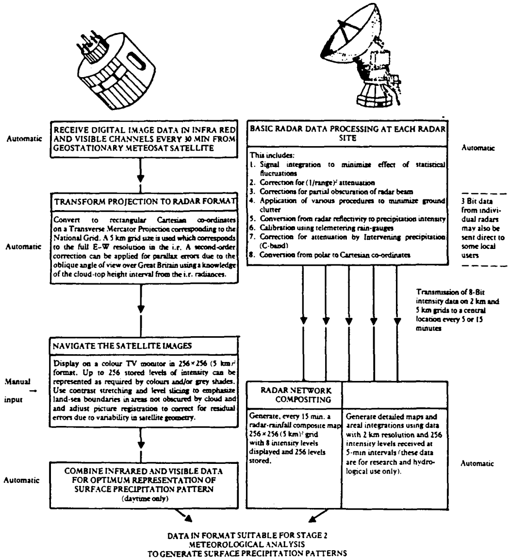
Fig. 16. Preprocessing of satellite and radar data for the "FRONTIERS" plan to use radar and satellite imagery for very short-range precipitation forecasting. (From Browning, 1979.)
