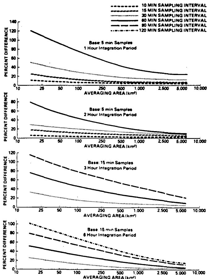
Fig. 8. Upper two panels: Mean absolute percent difference between rainfall estimates using 5-min base sampling intervals and those using coarser sampling intervals for a range of spatial averaging and temporal integration scales. Lower two panels: Same as upper two, except a 15-min base sampling interval was used and longer integration periods were included. Based on analysis by Hudlow and Arkell (1978), who used digital radar data collected over the eastern tropical Atlantic Ocean during the GARP Atlantic Tropical Experiment (GATE).
