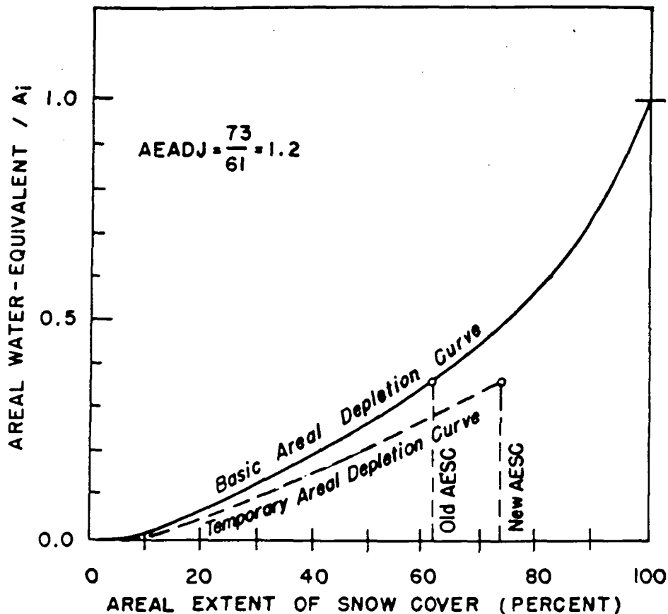
Fig. 19. Example of the effect of adjustment of the areal extent of snow cover on an areal depletion curve. AESC is Areal Extent of Snow Cover. AEADJ is the Areal Extent of snow ADJAdjustment factor. A_i is the minimum water-equivalent of the snow existing on a basin when the areal extent of snow cover reaches 100 per cent (Anderson, 1973).
