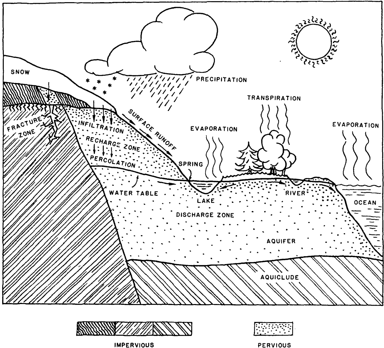
Fig. 23. Schematic cross-section showing occurrence of groundwater
