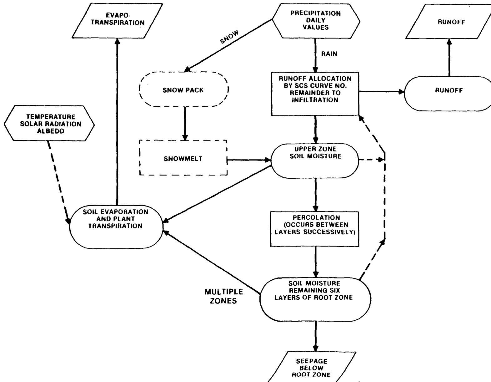
Fig. 21. Chemicals, Runoff and Erosion from Agricultural Management Systems (CREAMS) model option 1 schematic diagram (Peck et al., 1981).
