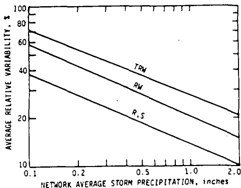
Fig. 9. Relations between relative variability and precipitation type on a 400 mi 2 network in central Illinois (from Changnon and Huff, 1980, p. 40). TRW = thunderstorm cases; RW = rain shower cases; R,S = continuous rain and snow cases.
