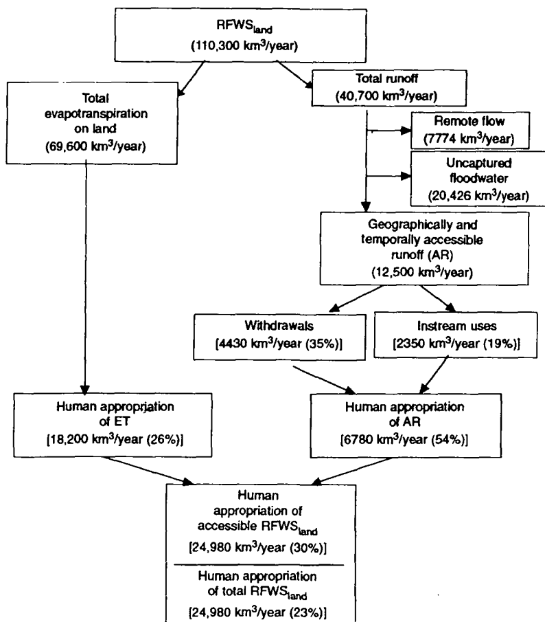
Fig. 2. Flow diagram of analysis of human appropriation of RFWS land . The final box shows human appropriation of estimated accessible RFWS land to be 30% (24,980 km 3 /81,100 km 3 ) and human appropriation of total RFWS land to be 23% (24,980 km 3 /110,300 km 3 ).
